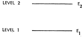
FIG. 1. Energy-level diagram for a two-level atom.
